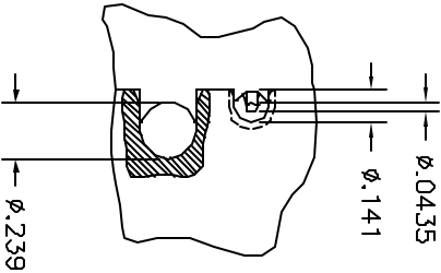
GAGING DIMENSIONS
